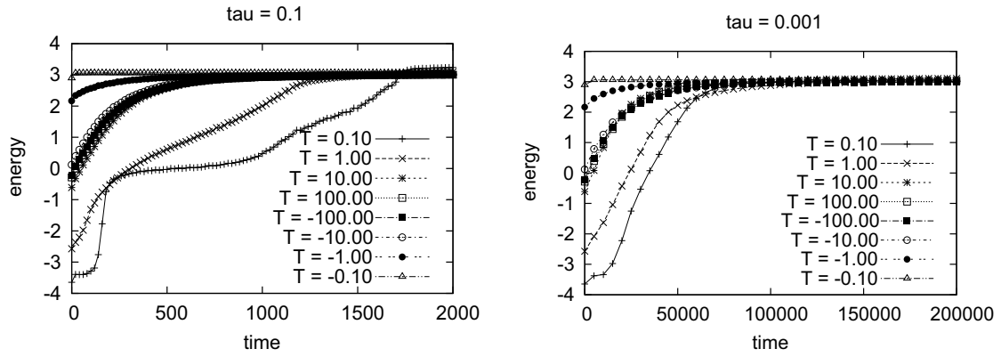
Fig. 1. Energy of the state as function of time for \beta = 1.0 with \tau = 0.1 (left) and \tau = 0.001 (right). Shown is the time evolution of an initially thermalized state (maximal entropy, Gibbs distribution, see text) in a lattice with N = 32 sites for a given temperature T = -100 \dots 100 .
