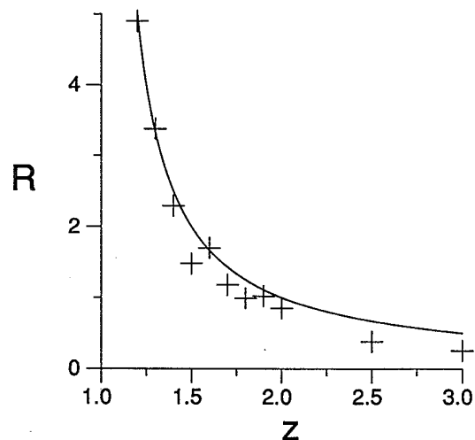
FIG. 4. Comparison of the diffusion indices for q=10 with the theoretical prediction (10).
