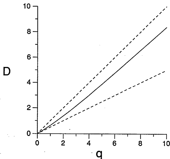
FIG. 5. The diffusion indices for the separatrix mapping (11).
