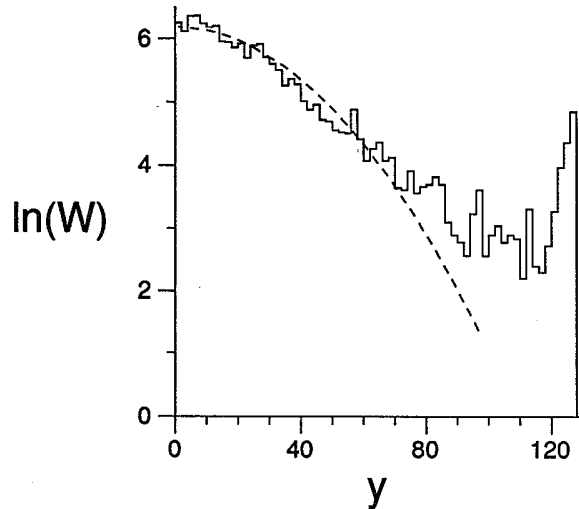
FIG. 3. The logarithm of probability distribution W(y,t) for t=128 . The dashed line approximates the main part of the distribution by the Gaussian law.
