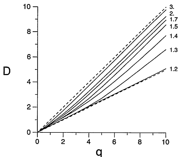
FIG. 2. The diffusion indices obtained for the mapping Fig. 1 for z ranging from 1.2 to 3. The dashed straight lines have slopes \frac{1}{2} and 1.
