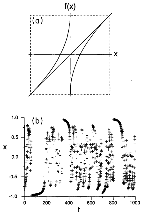
FIG. 1. (a) The Lorenz-type mapping and (b) the intermittent motion, produced by it.
